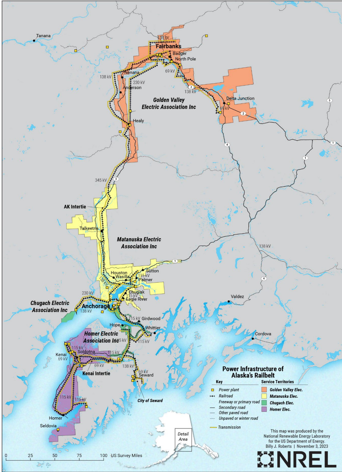
Figure 7. Power infrastructure of Alaska's Railbelt Grid Illustration by Billy J. Roberts, NREL
